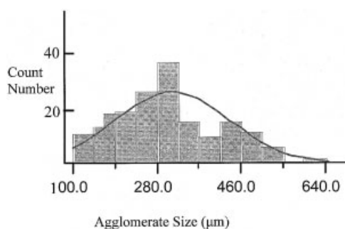
Figure 5. Typical agglomerate size distribution. Degussa Aerosil® R974.
